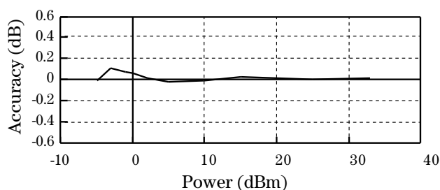
Power measurement accuracy +32 to -5 dBm
