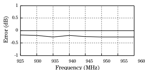
Typical RF generator RF in/out level error at -104 dBm
