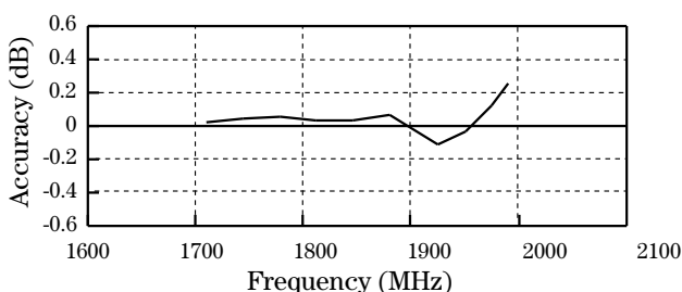
Power measurement accuracy 1710 to 1990 MHz
